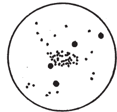
4. Andromeda galaxy
