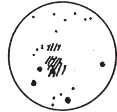
3. M41
