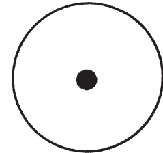
2. \epsilon Lyra
