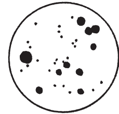
2. Orion Nebula
