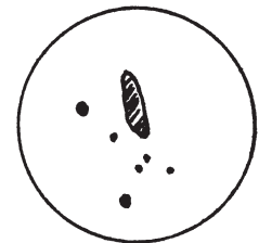
5. M52
