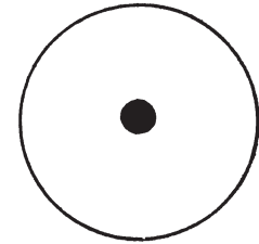
2. Hyades
