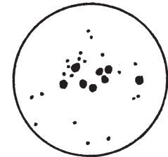
4. Andromeda galaxy
